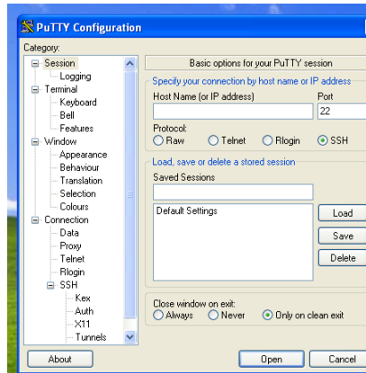
Fig. 1 Run PuTTY
