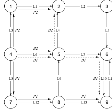
Figure 2. An example network topology
