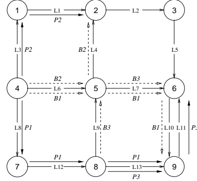
Figure 1. An example of backup multiplexing
