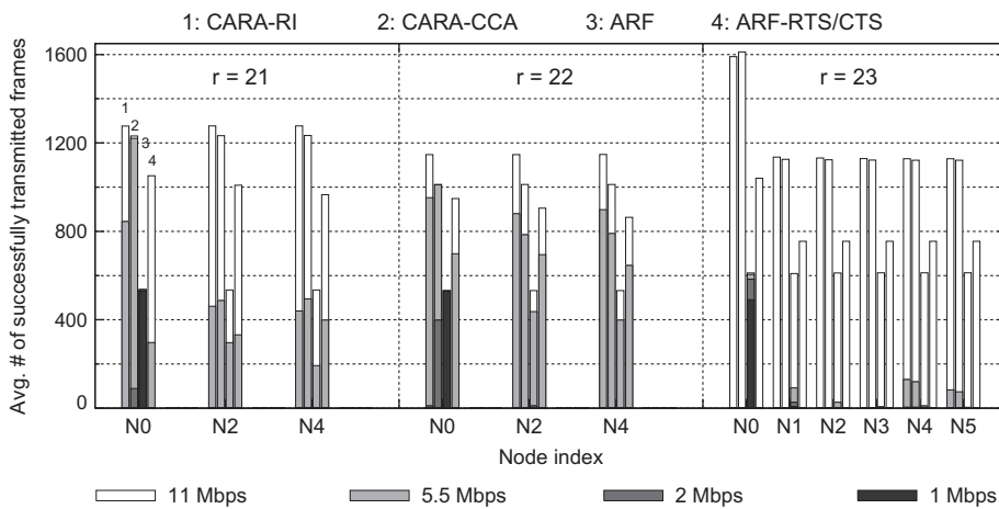
Fig. 9. Transmission rate distribution of the average number of successfully transmitted frames at each station; each bar shows the distribution of used rates and each scheme is enumerated as 1: CARA-RI, 2: CARA-CCA, 3: ARF, and 4: ARF-RTS/CTS.
