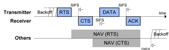
(b) RTS/CTS channel access mechanism.
