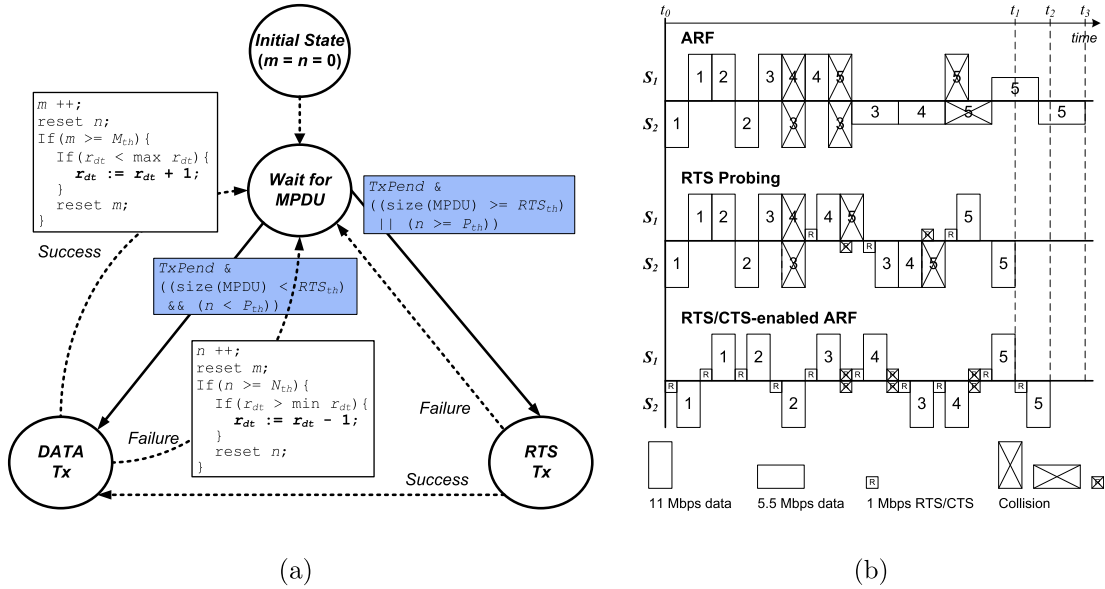
Fig. 2. (a) The state transition diagram of RTS Probing and (b) an illustrative example of ARF, RTS/CTS-enabled ARF, and RTS Probing timelines for a two-station 802.11b network, where the channel state is good enough to accommodate the highest rate of 11 Mbps.
