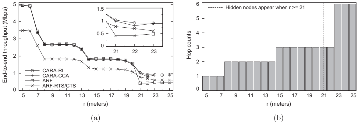
Fig. 8. Performance comparison in chain topologies with varying adjacent station distance ( r ): (a) throughput comparison of CARA schemes and ARF with/without RTS/CTS and (b) corresponding hop counts that are identical for all schemes as the ETT-based optimal route selection is commonly used.
