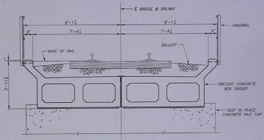
STRUCTURE NO. 5.4 - APPROACH SPANS
