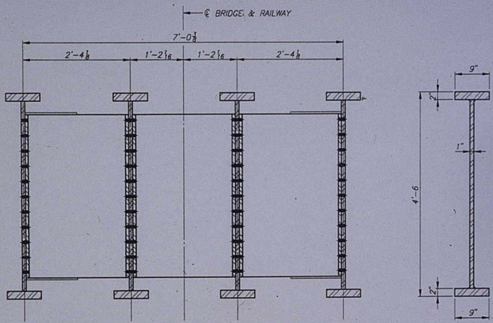
STRUCTURE NO. 3.1 - MAIN SPAN
